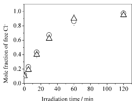
Figure 8. Mole fraction of free chloride ions [defined as (n_f)/(n_c + n_f) , where n_f denotes the number of moles of free chloride ions and n_c denotes the number of moles of chloride ions coordinated to ruthenium ion] for Ib ( \Delta ) and IIb ( \circ ) released during irradiation ( \lambda_{\text{irr}} in the range 400–600 nm; T = 20^\circ\text{C} ).
