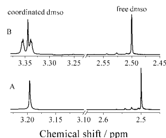
Figure 2. 1 H NMR spectra for trans -[RuCl 2 (dmso) 4 ] (A) and cis -[RuCl 2 (dmso) 4 ] (B) immediately after dissolution in CD 3 CN solution (for the trans isomer, the ratio of the integration area of the peak at 3.20 ppm to that at 2.50 ppm is 1:1; for the cis isomer, the ratio of the integration area of the peaks at 3.35–3.34 ppm to that at 2.50 ppm is 3:1); T = 20 °C.
