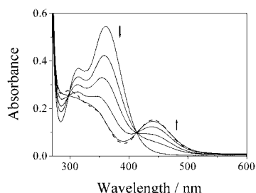
Figure 1. UV/Vis absorption spectra for a 1-mm dmso solution of cis -[RuCl 2 (dmso) 4 ] irradiated at 365 nm at room temperature for 0, 0.5, 1, 2, and 5 min; the dashed line denotes the spectrum of trans -[RuCl 2 (dmso) 4 ] in dmso solution.
