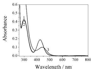
Figure 3. UV/Vis absorption spectra for a 1-mm acetonitrile solution of trans -[RuCl 2 (dmso) 4 ] recorded immediately after dissolution (1), after 15 min at 20 °C (2), and upon irradiation at \lambda_{irr} > 400 nm for 15 min (3); T = 20 °C.
