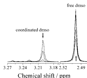
Figure 4. 1 H NMR spectra for trans -[RuCl 2 (dms o ) 4 ] (CD 3 CN solution) before irradiation (the ratio of the integration area of the peak at 3.20 ppm to that at 2.50 ppm is 1:1) and after being irradiated for 1, 5, and 15 min at \lambda_{\text{irr}} > 400 nm; T = 20 °C.
