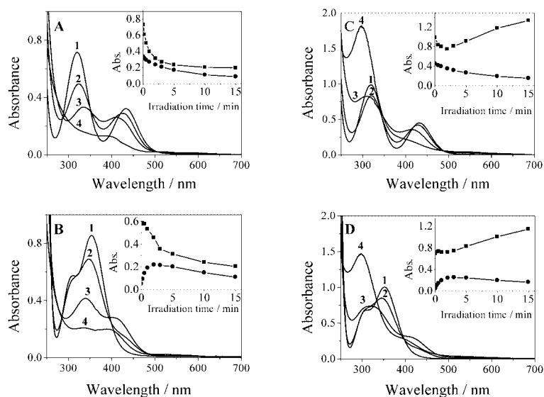
Figure 5. UV/Vis spectral changes during the photolysis ( \lambda_{\text{irr}} in the range 400–600 nm) of 2-mM aqueous solutions of Ib (A) and IIb (B) in an argon-saturated solution, and Ib (C) and IIb (D) in an air-saturated solution at room temperature. Spectra recorded after irradiation times of: 0 (1), 0.5 (2), 3 (3), and 15 min (4); T = 20^\circ\text{C} . Insets: absorbance against irradiation time at 320 (■) and 432 nm (●).
