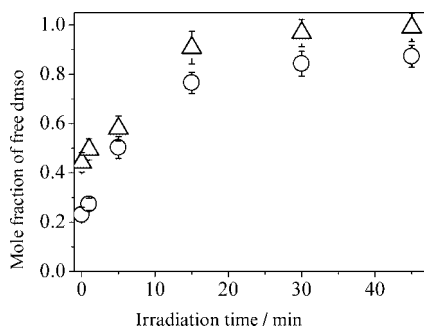
Figure 7. Mole fraction of free dmsO molecules [defined as (n_f)/(n_c + n_f) , where n_f denotes the number of moles of free dmsO and n_c denotes the number of moles of dmsO coordinated to ruthenium ion] for Ib ( \Delta ) and IIb ( \circ ) released during irradiation ( \lambda_{\text{irr}} in the range 400–600 nm; T = 20^\circ\text{C} ).
