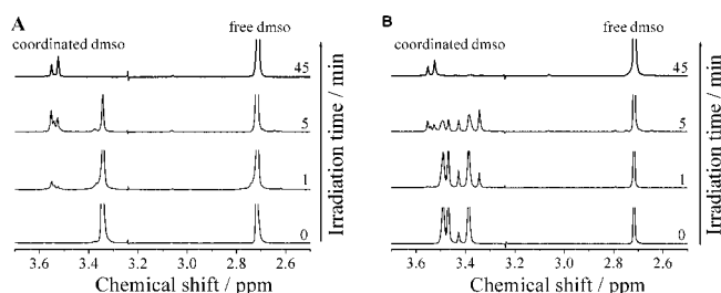
Figure 6. ^1\text{H} NMR spectra of the complex Ib (A) and IIb (B) ( \text{D}_2\text{O} solution) at various irradiation times; \lambda_{\text{irr}} > 400 nm, T = 20^\circ\text{C} .
